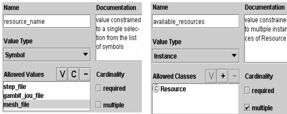
Figure 1 Protégé constraints on slot value
